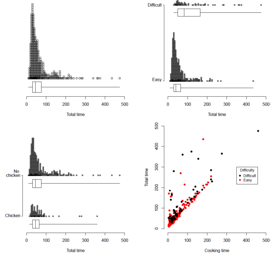
Figure 4: Exploratory data analysis for Total time
