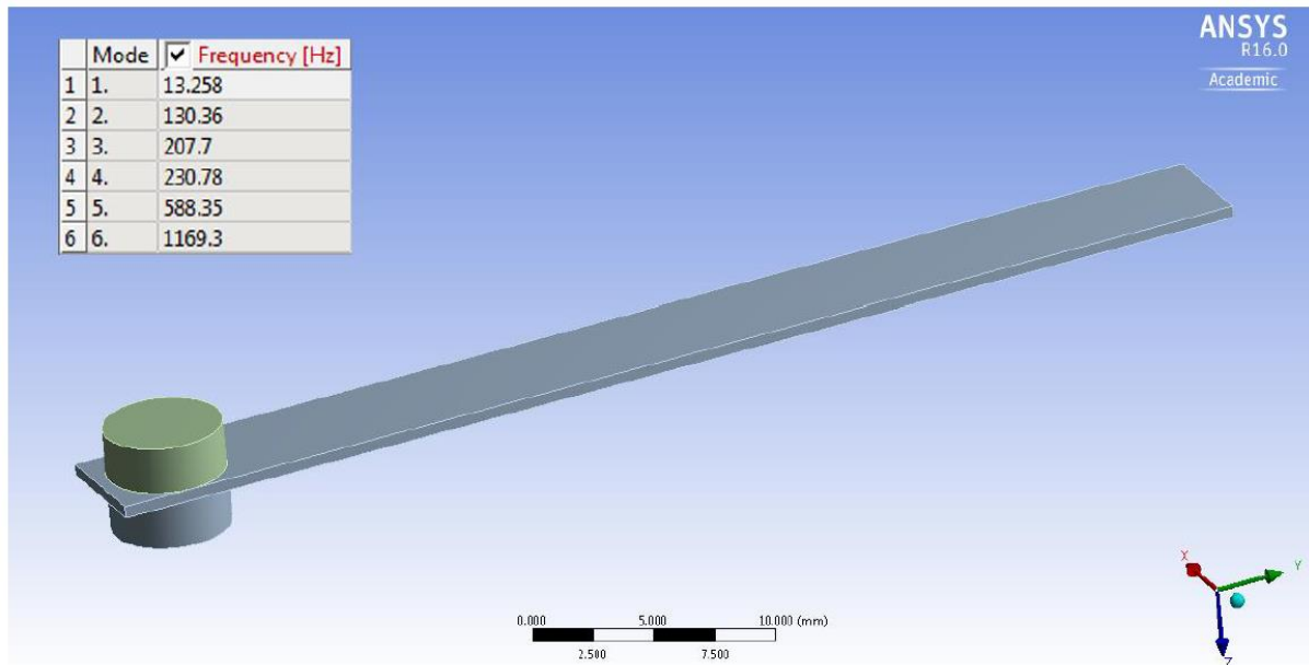
Figure 4 – ANSYS modelling of the cantilever to calculate its resonant frequencies
